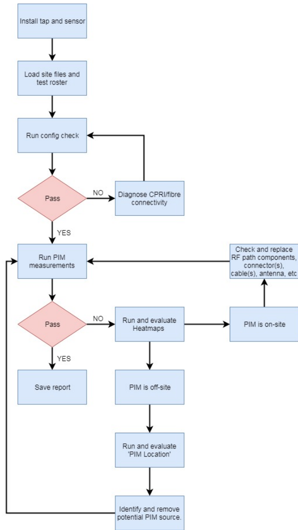
FIGURE 3 – PIM over CPRI (PIMForensics) PIM test set up
