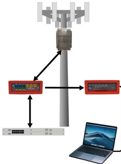
(PIMForensics) PIM test set up
