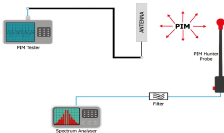
FIGURE 1 – RF-based PIM illustration
